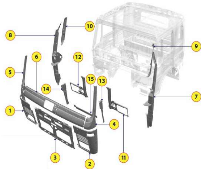
Cabin - Front Wall- 1
